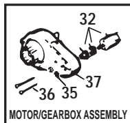
ASSEMBLY A
